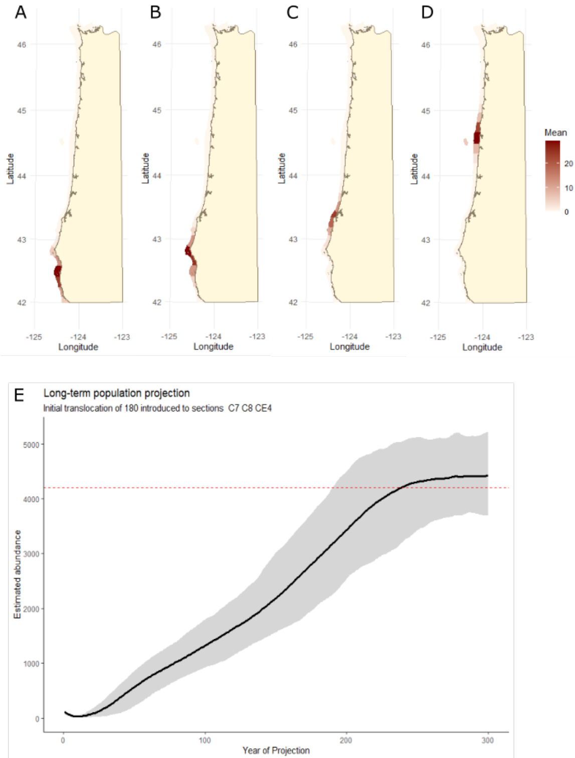
Figure 3.8. Simulation results from the ORSO population model associated with 4 alternative reintroduction scenarios (refer to Table 3.1). Panels A – D show maps of the expected distribution and abundance (indicated by color intensity) of sea otters after 25 years, based on reintroductions of 180 otters at each of 4 areas: A) Rogue Reef/Crook Point; B) Pt. Orford/Cape Blanco; C) Cape Arago/Coos Bay; and D) Yaquina Bay/Otter Rock. Panel E shows the model-projected population trends over 300 years after a reintroduction at Yaquina Bay/Otter Rock, with regional abundance approaching coast-wide K (red dashed line) approximately 200 years after the initial reintroduction.
